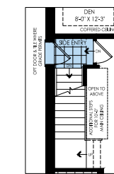
OPT. BASEMENT PLAN WALK-UP BASEMENT
